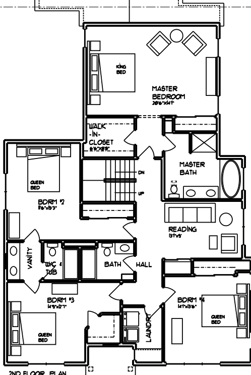
2ND FLOOR PLAN NO SCALE 1683 SF
